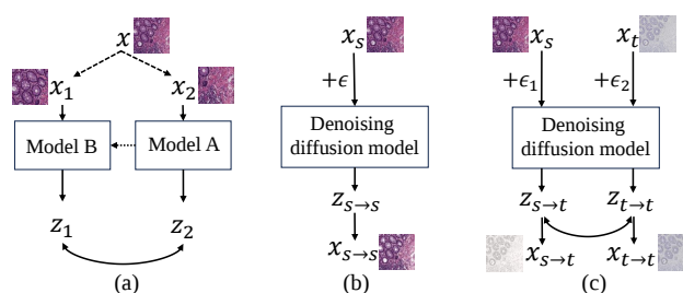
Figure 1: (a) Typical contrastive learning based pre-training framework. x_1 and x_2 are different views of input image x . (b) Denoising diffusion pre-training on image reconstruction task. \epsilon is the added noise. z_{s \rightarrow s} / x_{s \rightarrow s} denotes the reconstructed feature / image. (c) The proposed multi-modal denoising diffusion pre-training framework. z_{s \rightarrow t} and x_{s \rightarrow t} denote the re-stained feature and image generated in the re-staining task, respectively. z_{t \rightarrow t} / x_{t \rightarrow t} is the reconstructed feature / image in the reconstruction task.
